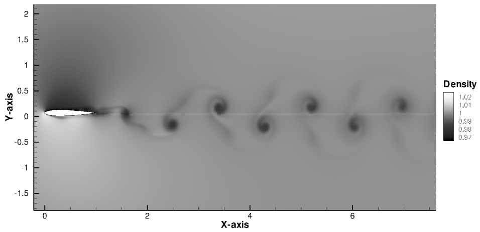
Figure 11. Vorticity field in the airfoil's wake - Sr = .60 , h = .2 , \tilde{k} = .3
