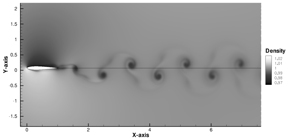
Figure 3. Density field in the airfoil's wake - Str = 0.29
