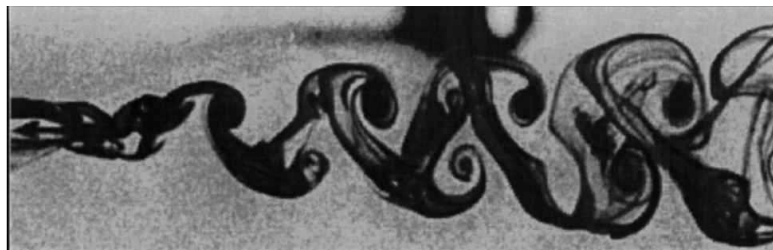
Figure 5. Streak lines, experimental data by Jones and Platzer - St = 0.29
