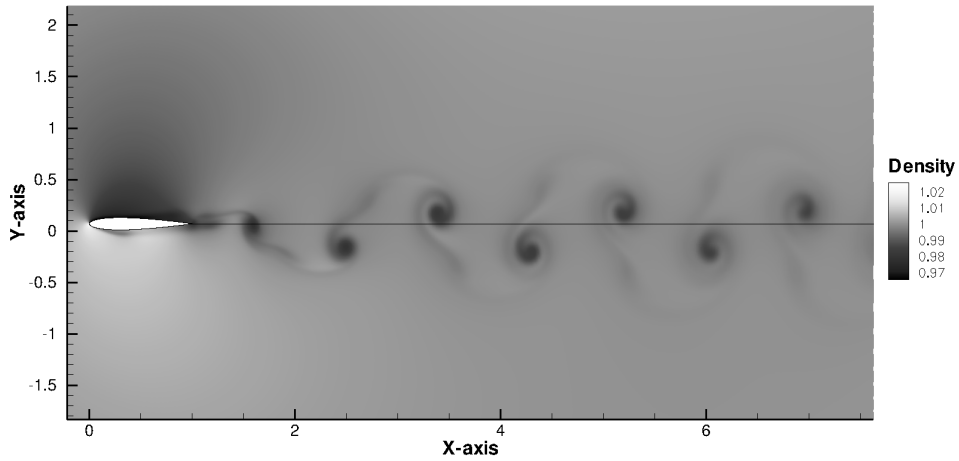
Figure 4. Vorticity distribution in the airfoil's wake - St = 0.29
