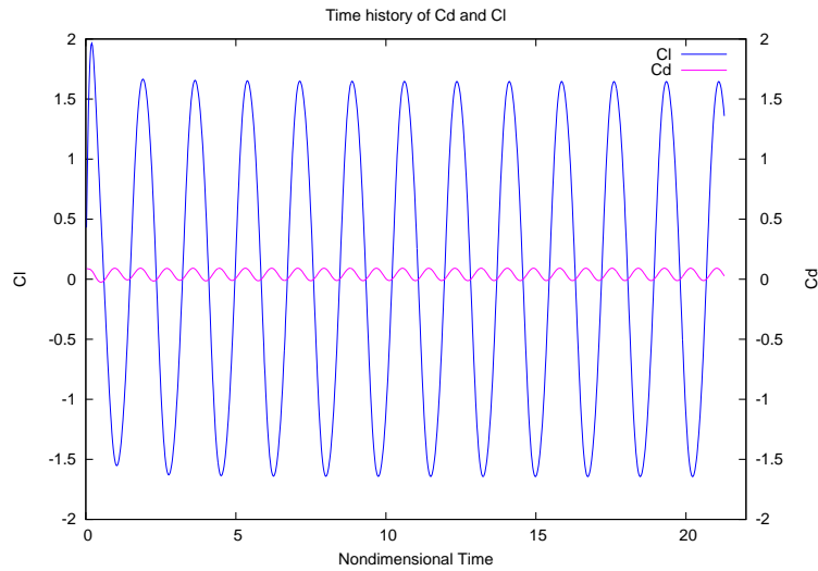
Figure 6. Lift and Drag history - St = 0.29
