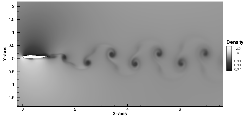
Figure 12. Density field in the airfoil's wake - Sr = 1.5
