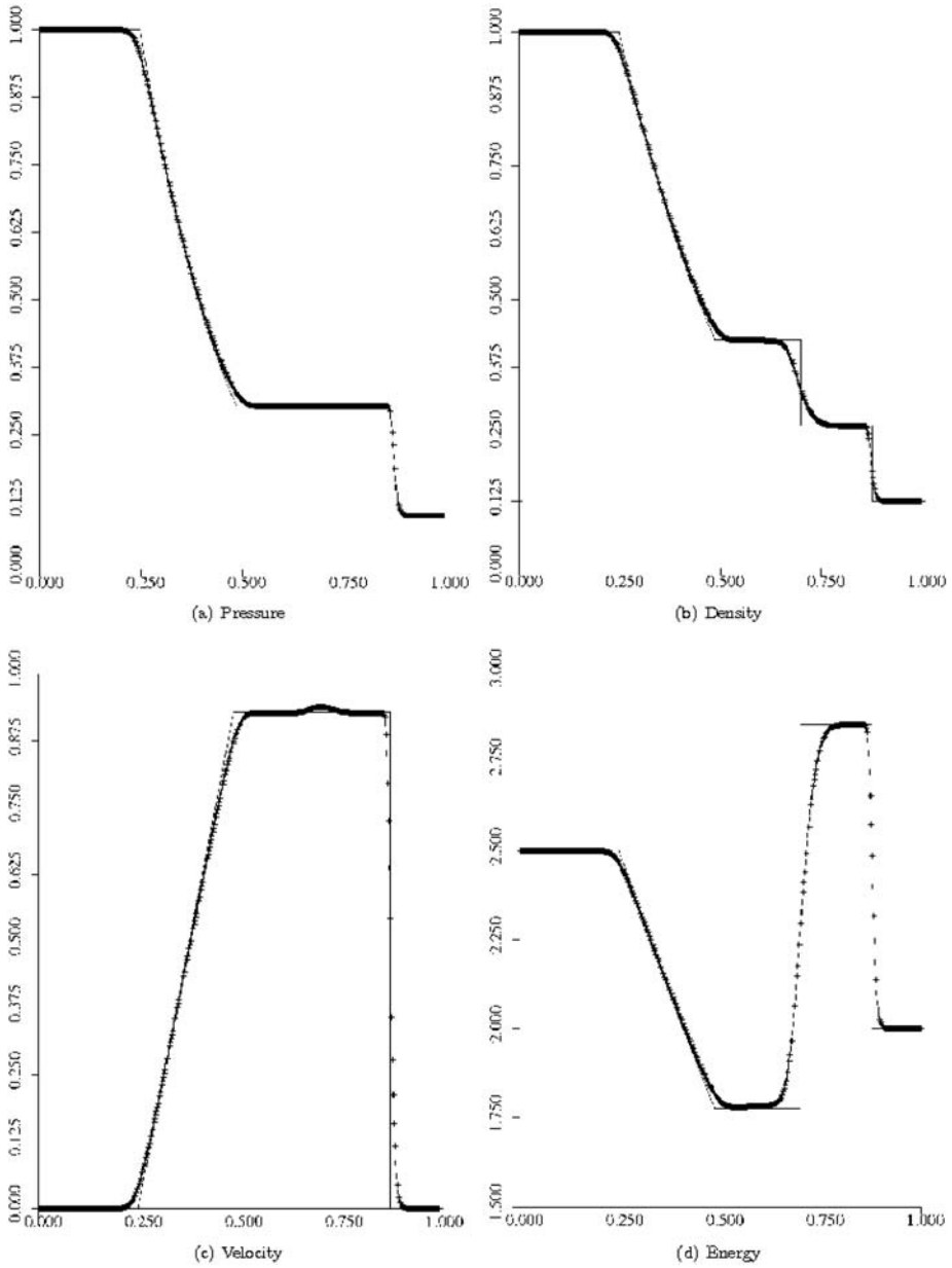
Fig. 6 Kinetic energy preserving scheme (coarse mesh): 512 mesh cells, Reynolds number 2500, computed solution values +, exact inviscid solution –
