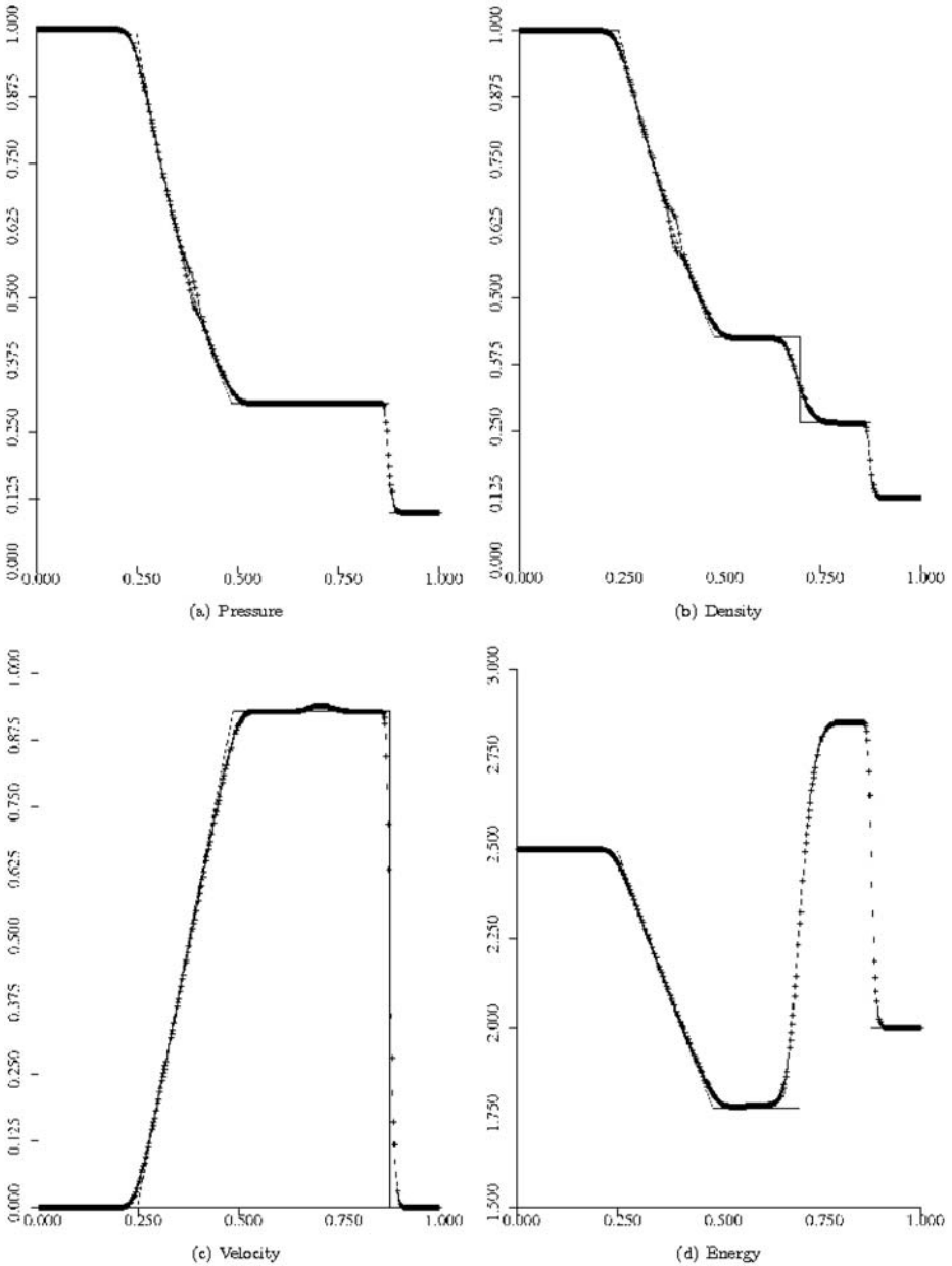
Fig. 4 Simple averaging of the flux (coarse mesh): 512 mesh cells, Reynolds number 2500, computed solution values +, exact inviscid solution –
