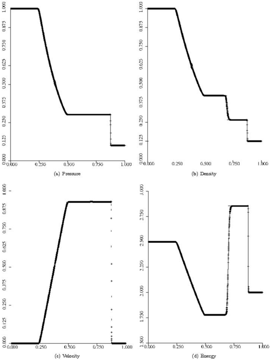
Fig. 1 Simple averaging of the flux: 4096 mesh cells, Reynolds number 25000, computed solution values +, exact inviscid solution –
