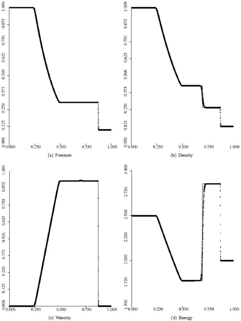
Fig. 3 Kinetic energy preserving scheme: 4096 mesh cells, Reynolds number 25000, computed solution values +, exact inviscid solution –
