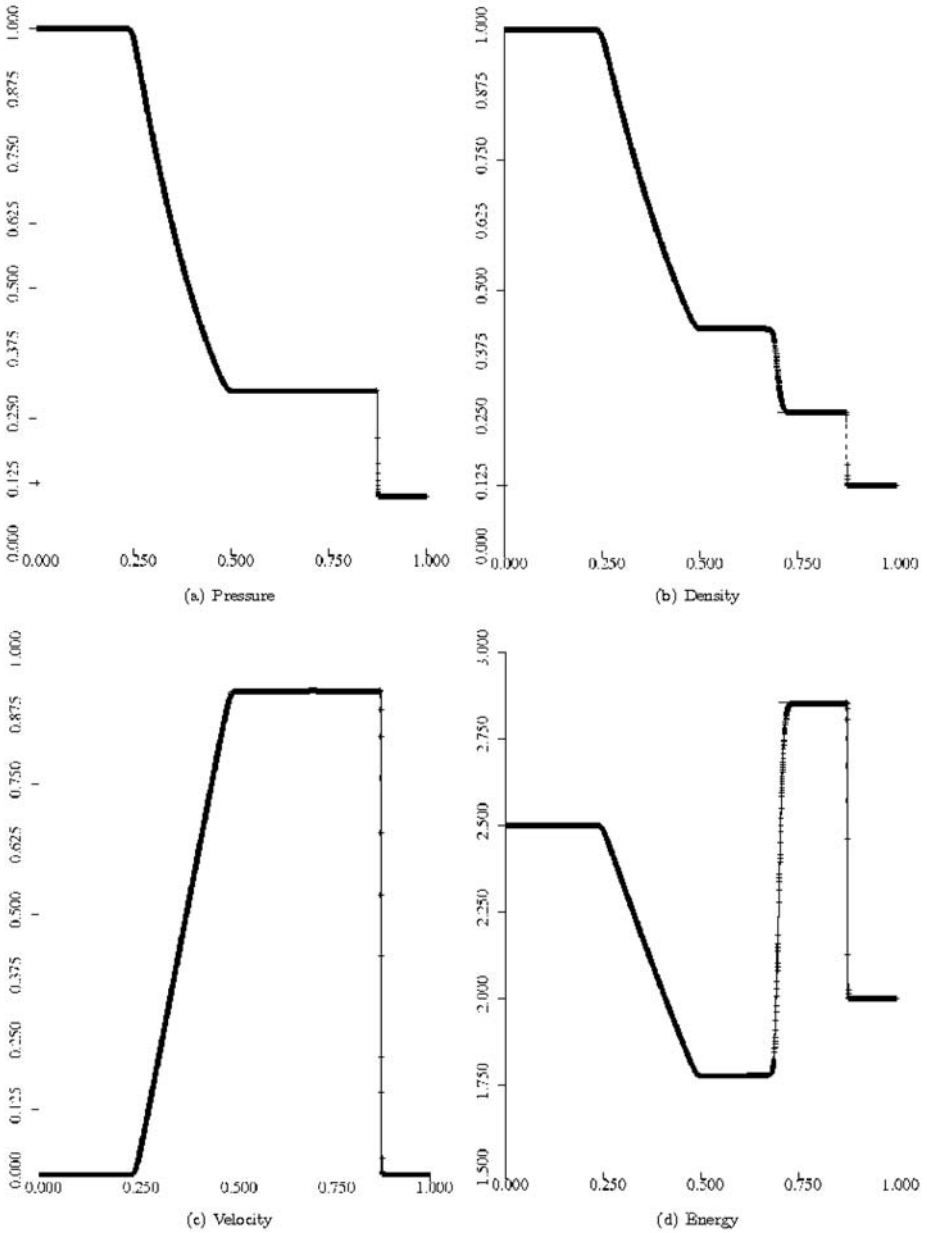
Fig. 2 Entropy preserving scheme: 4096 mesh cells, Reynolds number 25000, computed solution values +, exact inviscid solution –
