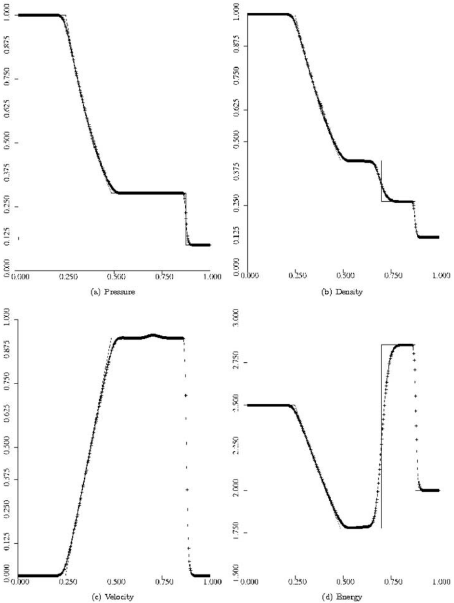
Fig. 5 Entropy preserving scheme (coarse mesh): 512 mesh cells, Reynolds number 2500, computed solution values +, exact inviscid solution –
