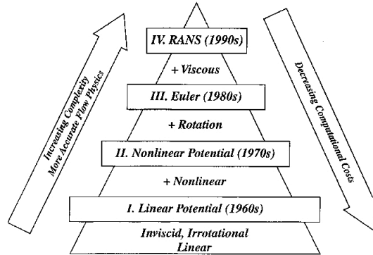
Figure 1: Hierarchy of models for industrial flow simulations
